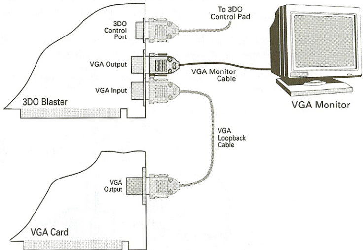
Figure 2-16: Connecting 3DO Blaster to VGA monitor.
